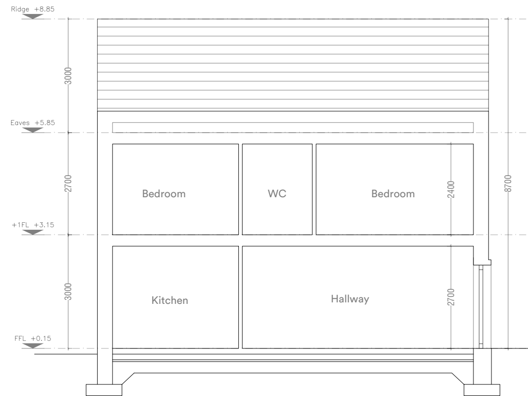
House Type N3 Semi-Detached Section A.A
